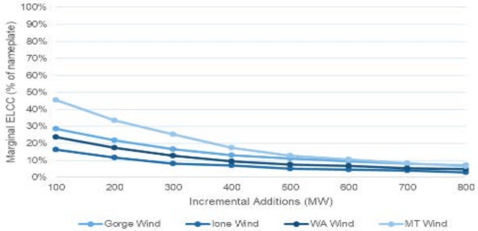
Figure 3-3 Marginal ELCC for wind resources Source: PGE 2019 Integrated Resource Plan 20
